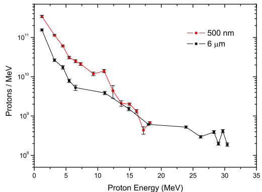
Figure 3: Experimentally obtained proton spectra, extracted from RCF stacks for 500 nm and 6 \mu\text{m} Al foil targets.
