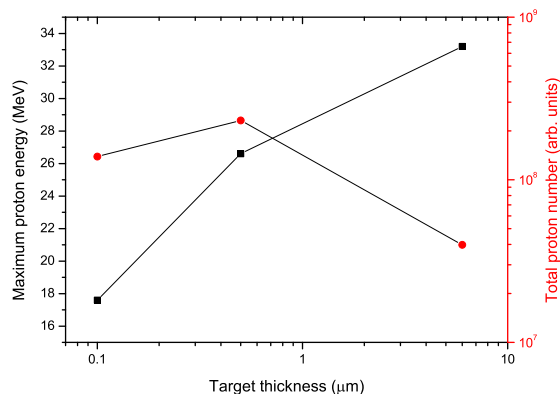
Figure 6: Maximum proton energies (squares) and integrated proton number (circles), as calculated from PIC simulations. Note: Proton number is sourced from macro-particles in the simulation and so given in arbitrary units.
