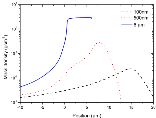
Figure 4: Simulated target density profiles at the point that the main laser pulse interacts with each target (laser is incident from the left hand side), modelling using HELIOS. The initial target front surface position is 0 \mu\text{m} .
