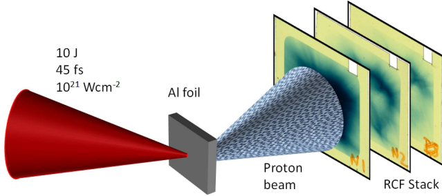
Figure 1: Overview of experimental set-up showing Astra-Gemini interaction beam and radiochromic film (RCF) stack. The RCF stack was positioned 45 mm from the rear surface of the target in order to capture the full proton beam.
