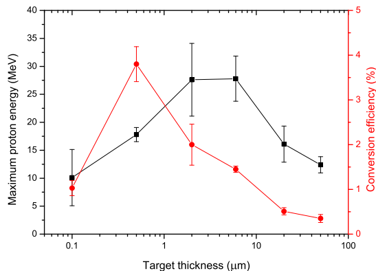
Figure 2: Maximum detected proton energy (squares) and conversion efficiency (circles, for E_p > 0.9 MeV) as a function of target thickness for Al foils. Data plotted are averages taken over a number of shots for each target thickness
