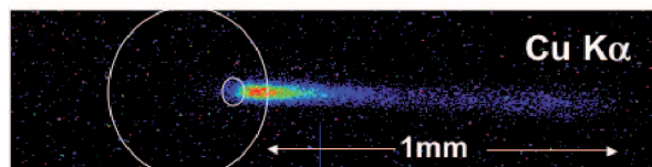
Figure 6. The K \alpha image and intensity line out of the cone wire target.
