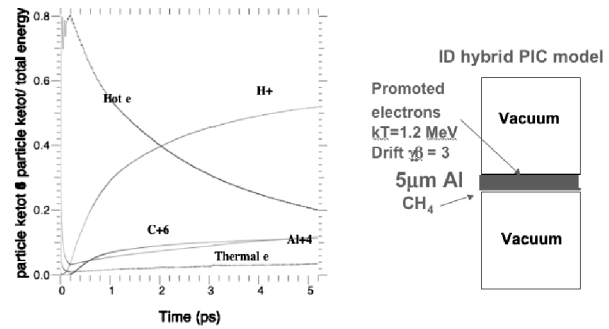
Figure 11. Hybrid PIC modeling of time evolution of energy components in 1D of conversion of hot electron energy in a 5 μm thick Al foil with 0.1 μm of CH 4 on the rear surface.
