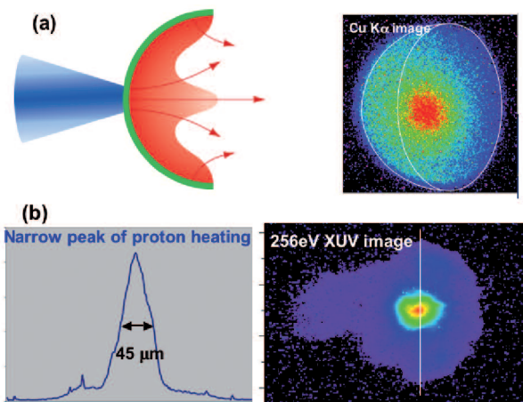
Figure 8. (a) Left: schematic sheath and proton plasma flow lines, (a) right: Kα image of 350 μm diameter Cu hemi-shell. (b) 256 eV image of focused proton heating of a polymer foil with associated XUV intensity line out.
