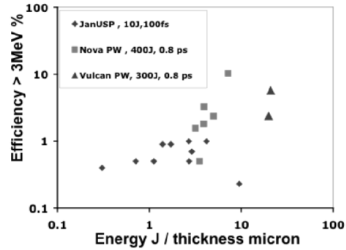
Figure 10. Collected data on conversion efficiency to >3MeV protons versus laser energy/target thickness.
