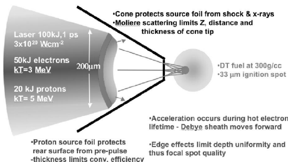
Figure 7. Conceptual proton fast ignition.
