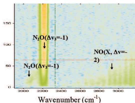
Figure 2. Contour plot of spectra recorded at a resolution of 20 \text{cm}^{-1} following pumping of NO(X) (total pressure: 500 mTorr) to its A state in the presence of 50 mTorr N_2O ( \Phi_{N_2O} = 0.07 ).
