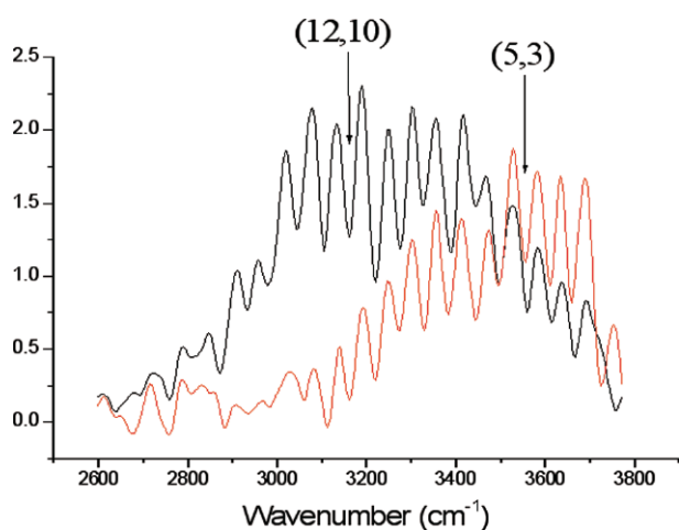
Figure 1. NO ( \Delta v' = -2 ) emission spectrum at 10 \mu s following irradiation of 50 mTorr of NO on its A state resonance in the presence of 3.5 Torr of N_2O ( \Phi_{N_2O} = 0.9 , red) and 5 Torr of NO ( \Phi_{NO} = 0.9 , black). Selected band origins have been shown.
