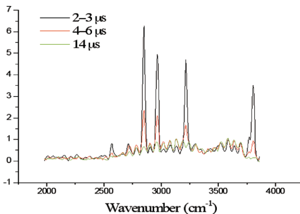
Figure 4. Emission spectra over time following the pumping of NO to its A state (total pressure: 50 mTorr) in the presence of 120 Torr of Xe ( \Phi_{Xe} = 0.5 ).
