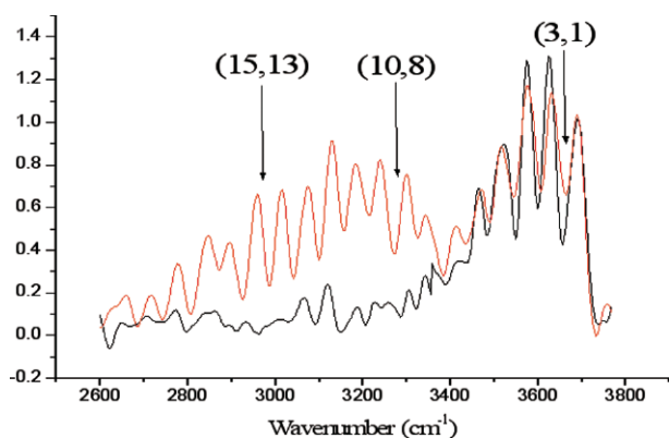
Figure 3. NO ( \Delta v' = -2 ) emission spectrum at 10 \mu s following 226 nm irradiation of 50 mTorr of NO(X) in the presence of 120 Torr of Xe ( \Phi_{Xe} = 0.5 , red). Also shown is self-quenching by NO, which has a Franck Condon distribution ( \Phi_{NO} = 0.1 , black). Selected band origins are shown.
