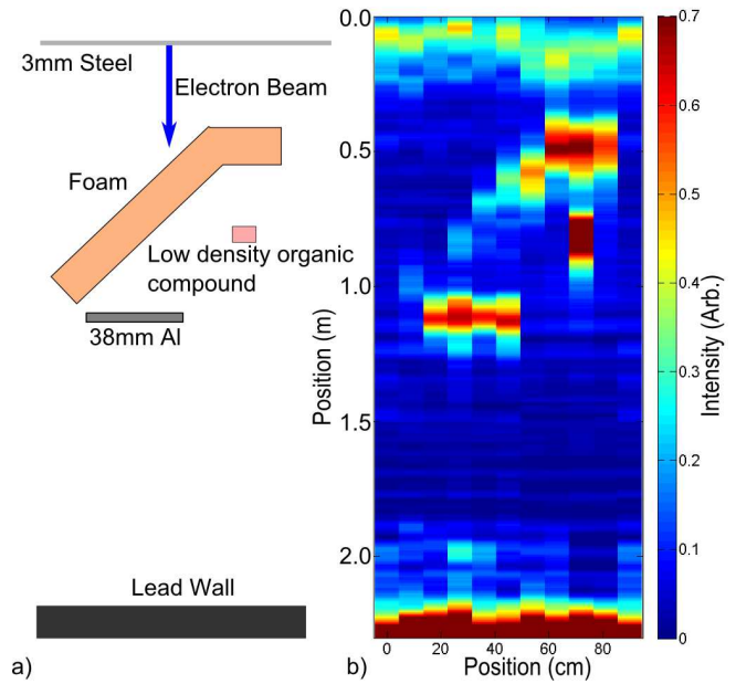
Figure 6: a) Diagram of the set-up of the array of test objects. b) Example of an X-ray backscatter image of the object array shown in a). An array of objects including 38mm thick Al, 0.14m thick insulation foam and a low density organic compound are shown.
