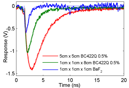
Figure 5: Comparison of output signal from BC422Q 0.5% plastic scintillators in a 50mm long 50mm diameter cylinder (red line), 10mm \times 10mm \times 80mm cuboid (green line) and 4 10mm \times 10mm \times 10mm BaF 2 crystals (blue line) with a 195nm bandpass filter. Data is averaged over 4, 5 and 10 shots respectively and the BaF 2 signal has been scaled up by a factor of 5 to allow comparison with the other signals. Dashed lines show curve fits assuming curve of the form \exp(-t/t_{decay}) - \exp(-t/t_{rise}) [16], where t_{decay} and t_{rise} are the decay and rise time constants.
