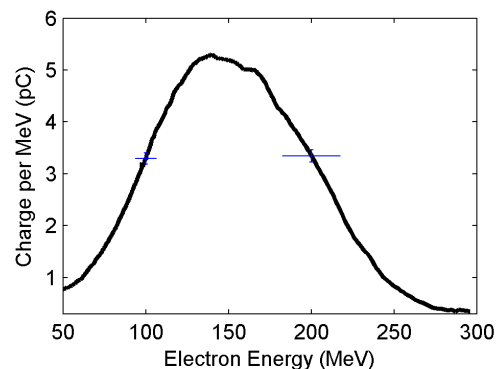
Figure 3: Electron spectrum measured on a Kodak Lanex screen. Electrons are produced with 3.9 \times 10^{18} \text{ cm}^{-3} He + 5% N gas jet and deflected a 100mm 0.67T magnet. Peak energy is shown to be approximately 140 \text{ MeV} \pm 10 \text{ MeV} with a 120MeV FWHM energy spread. Typical error bars for points at either end of the spectrum are shown. These errors are largely due to uncertainties in position measurements and the charge calibration.
