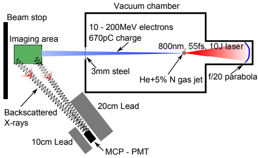
Figure 4: Plan view diagram of experimental set-up showing positions of MCP - PMT detectors, imaging samples, gas jet and electron beam.
