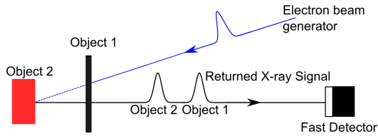
Figure 1: Schematic of electron generated X-ray backscatter detection.
